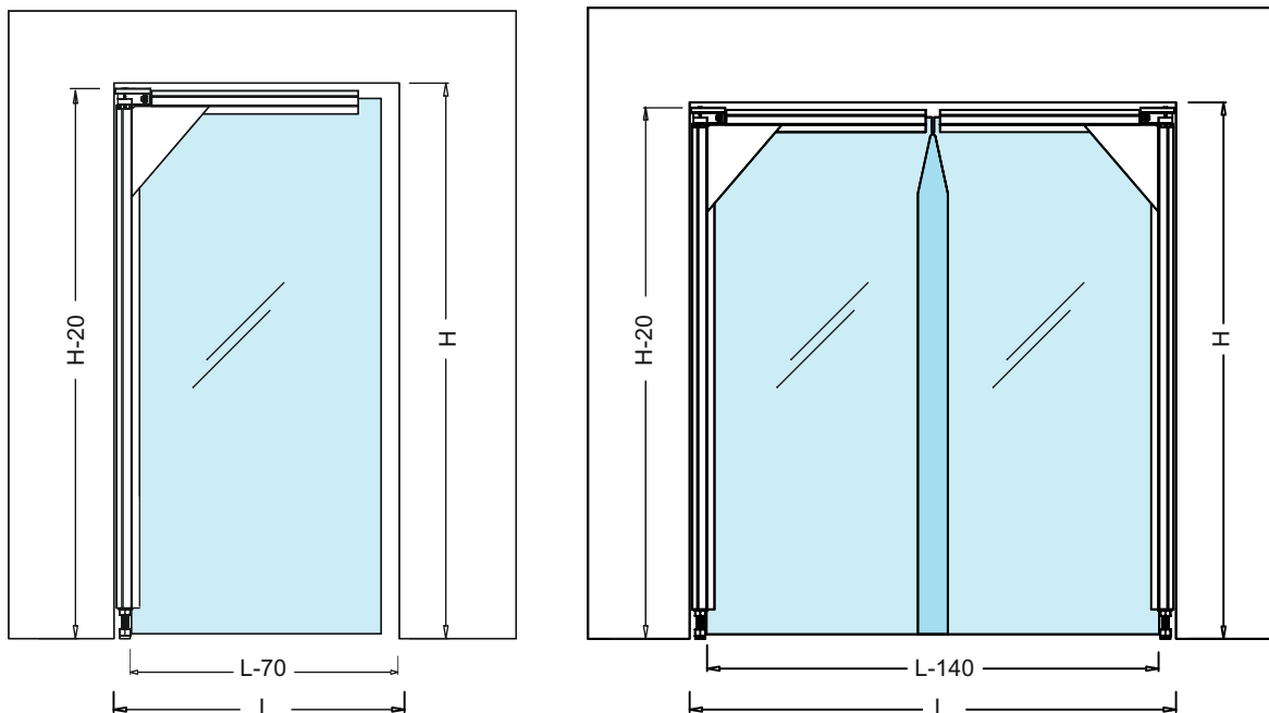
Flap 1A single blade flap door portes souples 1 vantail
